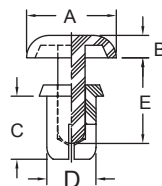
FIG. 2 十字头 Across slot
