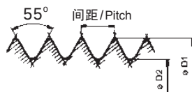
G型螺纹
