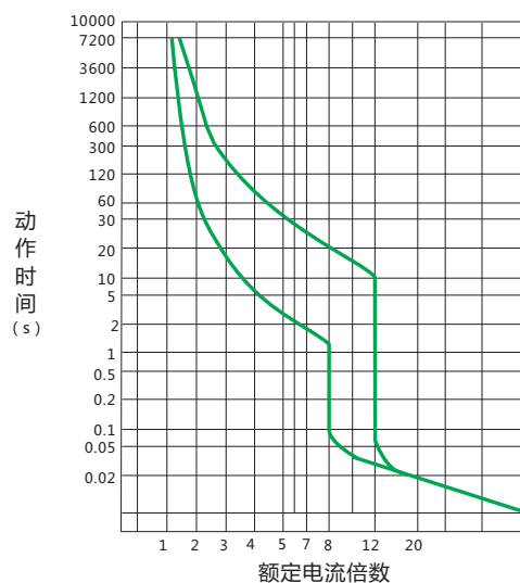
NXMLE-250
