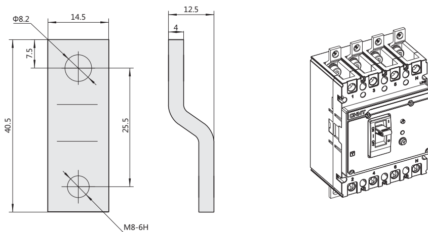
NXMLE-160S/H
