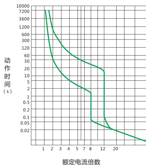
NXMLE-250
