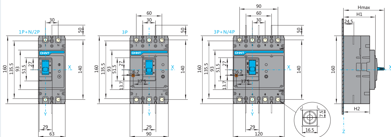
NXMLE-160S/H
